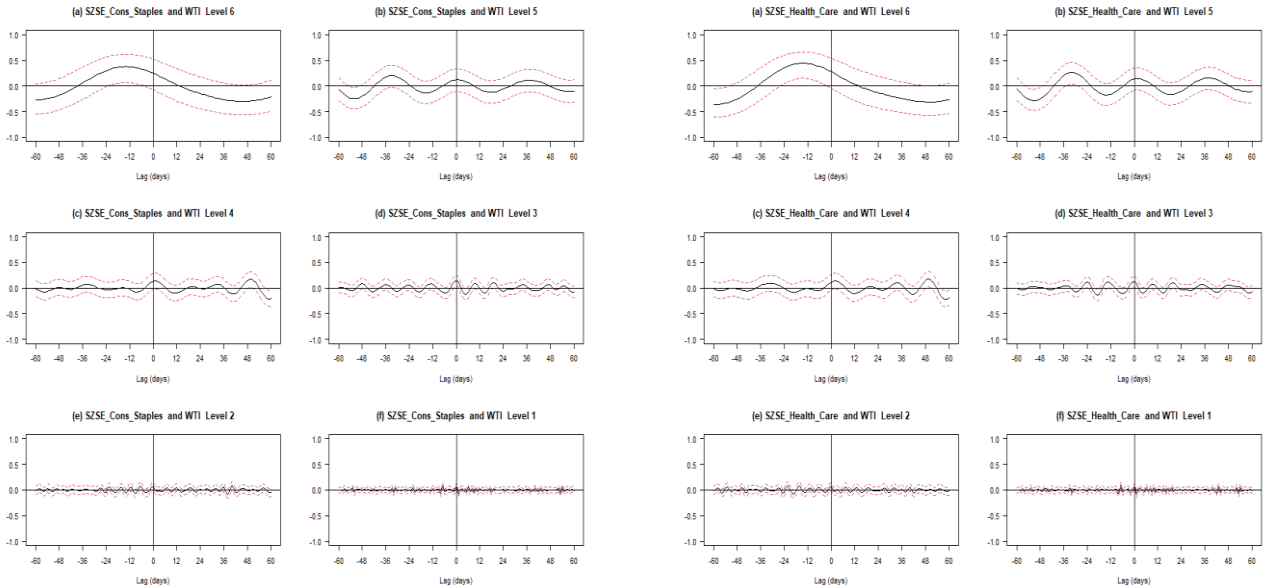
Figure 36 Cross-Correlation between SZSE Cons Staples and WTI at different time scales
